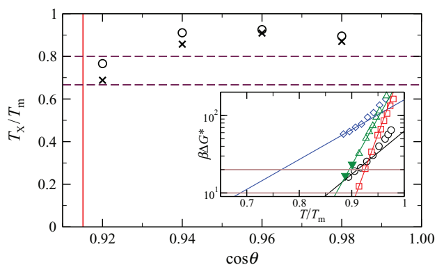
FIG. 11. Estimates of homogeneous nucleation temperature T_X^{10} (crosses) and T_X^{20} (circles) as functions of \cos \theta . The solid vertical line indicates the value of \cos \theta = 0.9151 at which more than one bond per patch becomes possible for \delta = 0.24 . The upper horizontal dashed line marks the approximate value of T_g/T_m = 0.8 for silica, while the lower one indicates the general value of T_g = 2T_m/3 . Inset shows the determination of T_X^{10} and T_X^{20} from the crossing of exponential fits to the four lowest T points for each value of \cos \theta with \beta\Delta G^* = 10 and 20 , respectively.
