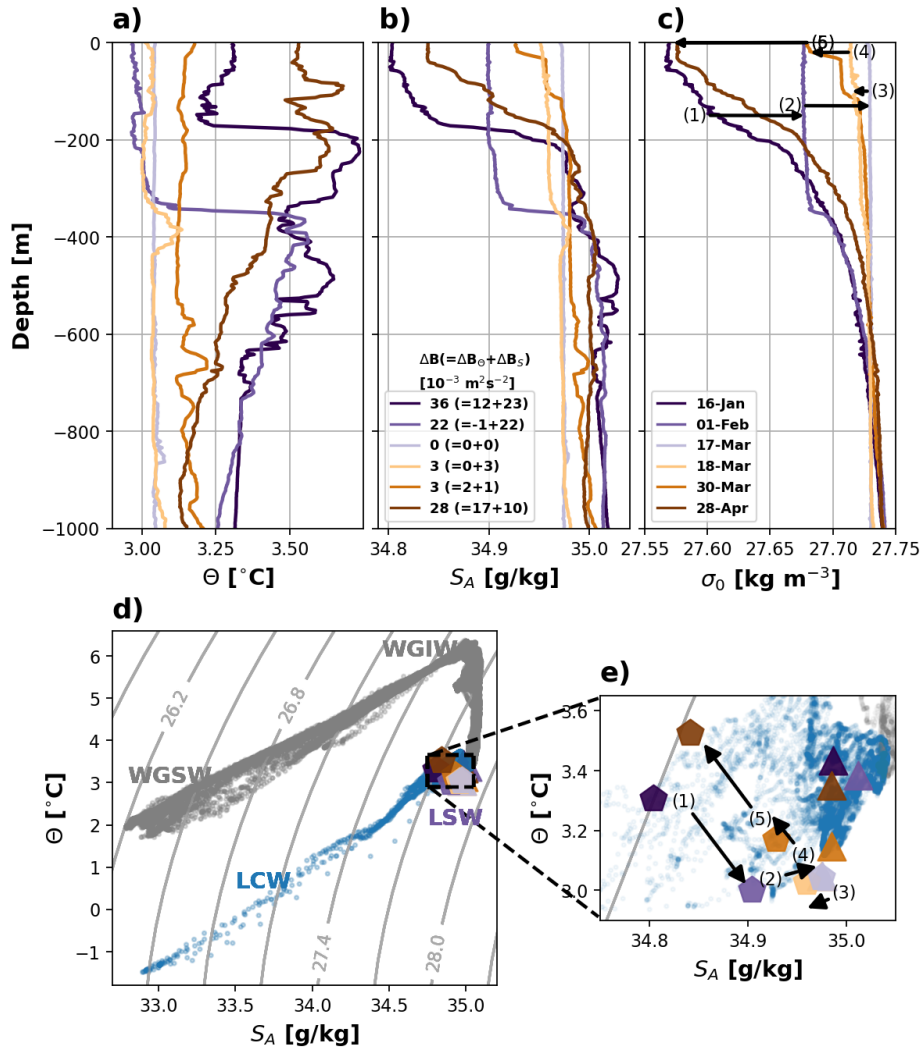
FIG. 6. Convection-restratification cycle at the deep convection region (PearlDiver) from January (dark purple) to April (dark brown) (a) in temperature, (b) salinity, (c) density, (d)/(e) and in \Theta - S_A space depth-averaged within (pentagon) or below (triangle) the ML. Buoyancy anomaly ( \Delta B ) with its \Theta and S_A components relative to the deepest convection (lightest purple) integrated over the top 400 m (legend in (b)). The \Theta - S_A properties of waters sampled inshore of the 2000 m isobaths by sg638 are added in (d)/(e): West Greenland Shelf Water (WGSW), West Greenland Irminger Water (WGIW), Labrador Current Water (LCW), and Labrador Sea Water (LSW).
