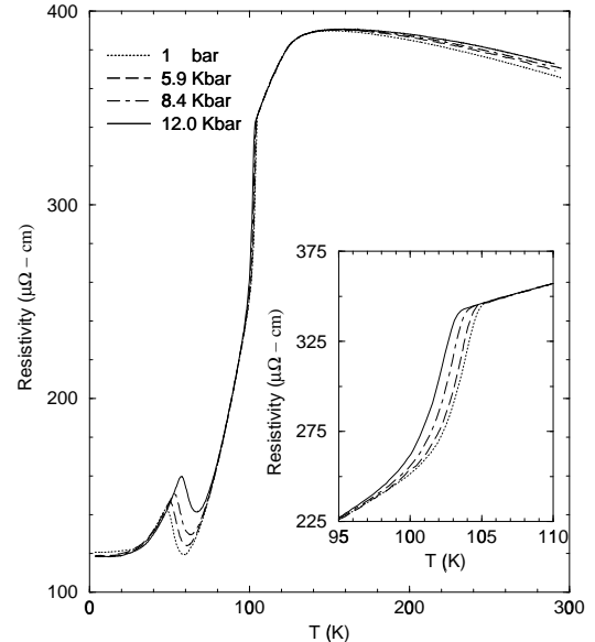
FIG. 2. Temperature dependence of the resistivity ( \rho_{\parallel} ) of \text{UNi}_2\text{Si}_2 with the current parallel to the c -axis for pressures: P = 1 bar, 5.9 Kbar, 8.4 Kbar and 12.0 Kbar. The inset magnifies the data to show more clearly the effect of pressure on the phase transition at 103 K.
