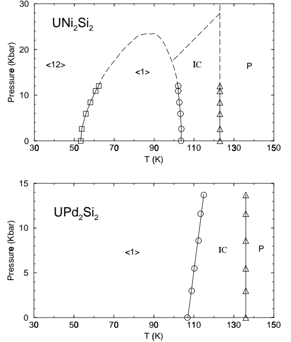
FIG. 3. Pressure-temperature magnetic phase diagram of \text{UPd}_2\text{Si}_2 and \text{UNi}_2\text{Si}_2 .
