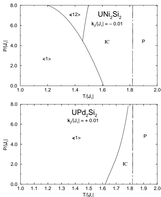
FIG. 4. Magnetic phase diagram with exchange parameters J_0 = 1 , J_1 = -1 , J_2 = -0.30 , and J_3 = 0.03 and k_2/|J_1| = +0.01 for \text{UPd}_2\text{Si}_2 and k_2/|J_1| = -0.01 for \text{UNi}_2\text{Si}_2 . Solid and broken curves represent first-order and continuous transitions, respectively. The AF phase is labelled as (1).
