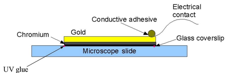
Figure 3.3: A schematic diagram of the substrate used in experiments for this thesis.
