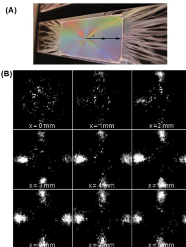
Figure C.1: Upon translation along the radial direction shown in (A), nine successive laser diffraction patterns were obtained (B). These diffraction data correspond to y = 0 \text{ mm} , obtained at 1 mm intervals from x = 0 \text{ mm} to x = 8 \text{ mm} . The sample was spin coated at 3000 rpm from a silica suspension in acetone.
