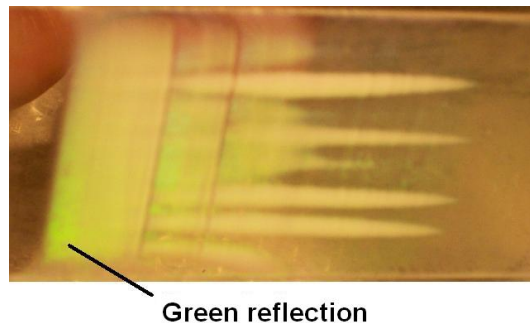
Figure 1.1: A colloidal crystal prepared by the dip-coating technique in our laboratory. The green color is due to Bragg reflections from a close-packed colloidal crystal.
